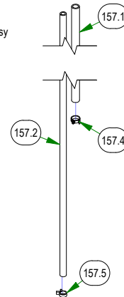
067-0020-01 ZT/Mav EPA Cannister Assy
