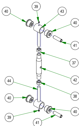
048-7000-00 Turnbuckle
