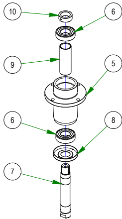
037-6015-50 Spindle- Aluminum -2012 ZT
