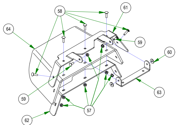
210-7000-98 2019 Outlaw Gen2 Chute Assembly
