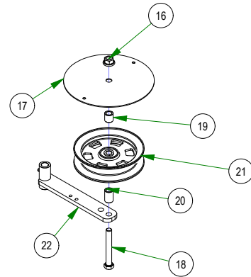
039-6945-20 2020 61 Revolt Deck Idler Assembly
