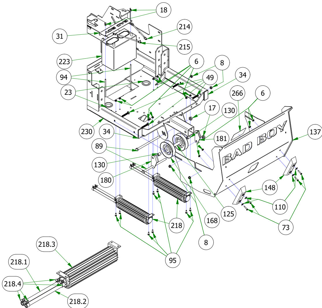
Oil Cooler Assembly
