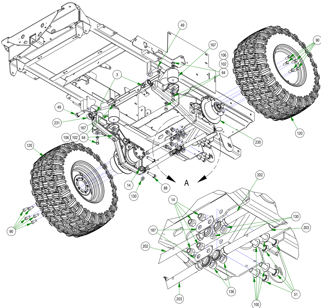
DETAIL A
