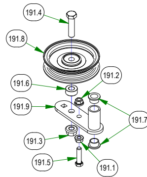
039-6950-94 RIGHT PUMP IDLER
