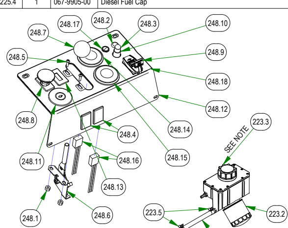
079-3480-22 CONTROL PANEL
